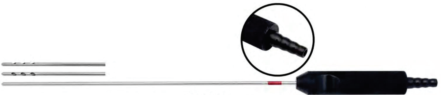
WI-SU-1760 RICHTER SUCTION TUBE ,DIA 4.0MM WITH 3 SUCTION HOLE 30CM WORKING LENGTH
