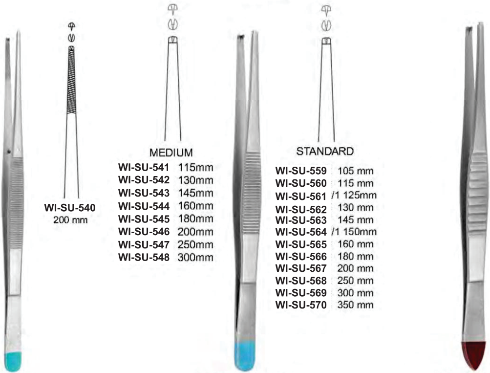
TISSUE FORCEPS 1X2 Teeth
